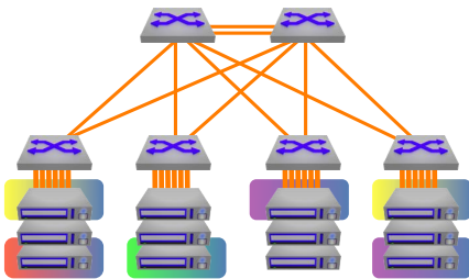
Arista Fixed System Leaf-Spine Designs Scale to 6,144 10GbE/25GbE ports or 1,536 40GbE/100GbE port at 3:1 subscription
